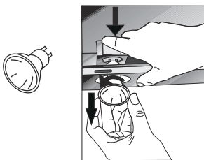
Fig. 18: Lamp Replacement
