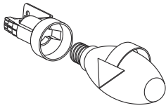
Fig. 19: Lamp Replacement
